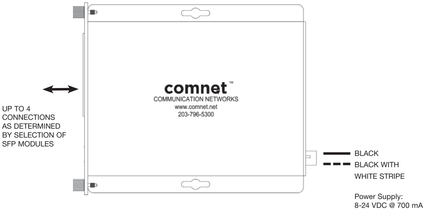
FIGURE 1 – CNGE4US UNMANAGED SWITCH
