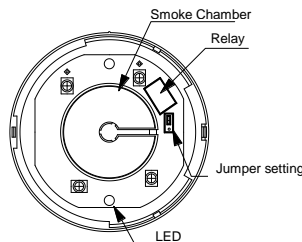
Figure 3. Schematic of detector structure When front cover is open.
