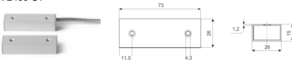
MK-2400-S1
